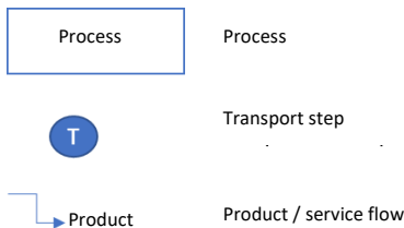
Figure 1: Hybris Lifecycle
