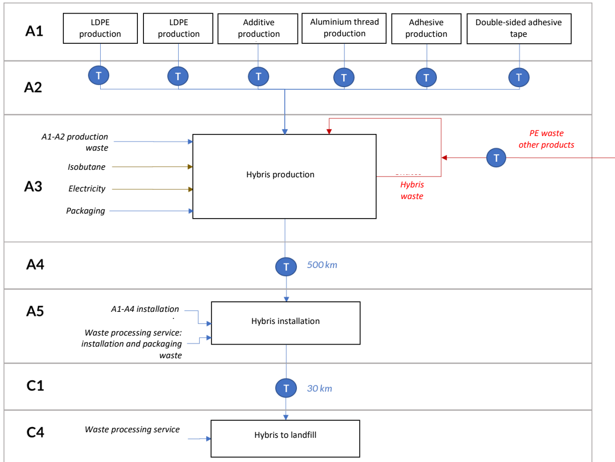
Figure 1: Hybris Lifecycle
